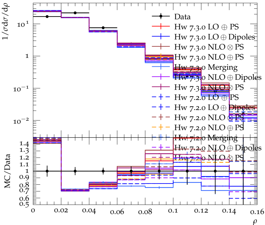
Scaled light jet mass at 43.5 GeV
