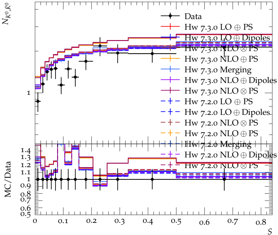
K^0, \bar{K}^0 multiplicity vs sphericity at 42.6 GeV
