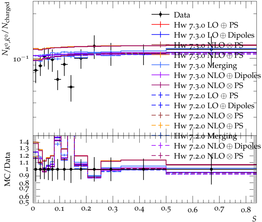
N_{K^0, \bar{K}^0} / N_{\text{charged}} vs sphericity at 42.6 GeV
