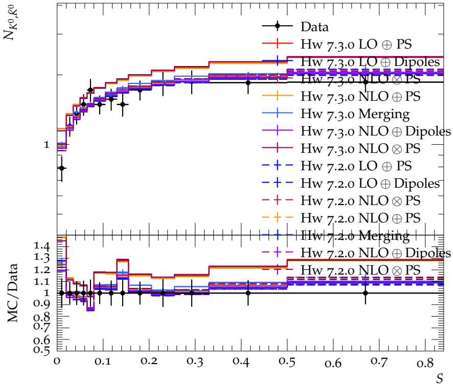
K^0, \bar{K}^0 multiplicity vs sphericity at 35.0 GeV
