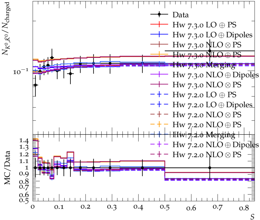
N_{K^0, \bar{K}^0} / N_{\text{charged}} vs sphericity at 35.0 GeV
