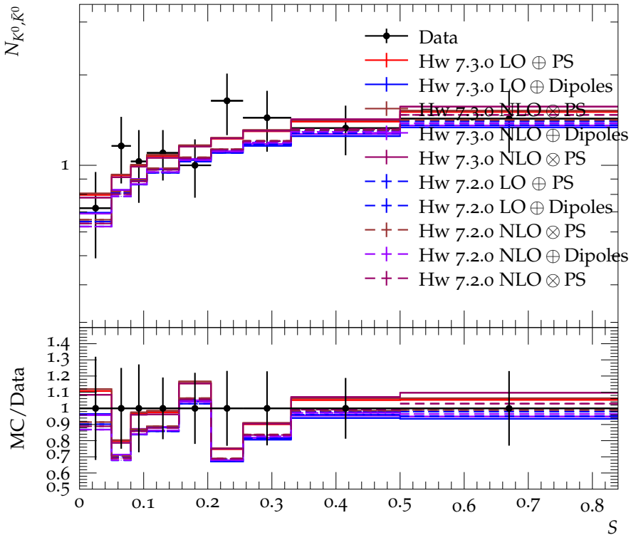
K^0, \bar{K}^0 multiplicity vs sphericity at 14.8 GeV
