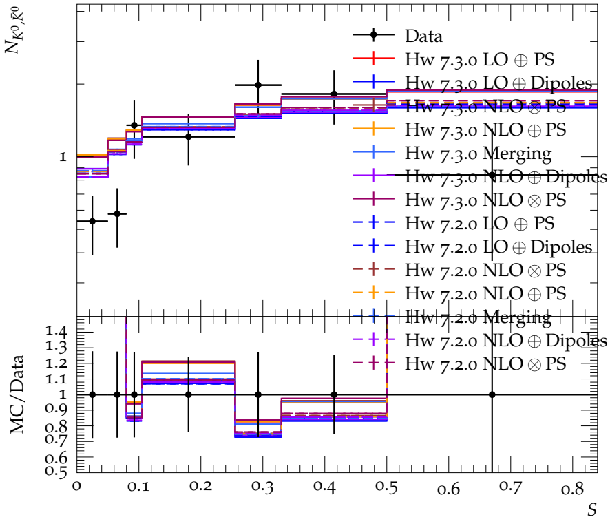
K^0, \bar{K}^0 multiplicity vs sphericity at 21.5 GeV
