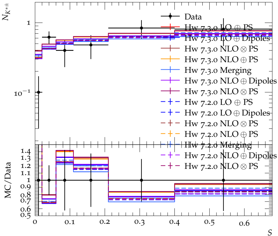
K^{*\pm} multiplicity vs sphericity at 35 GeV
