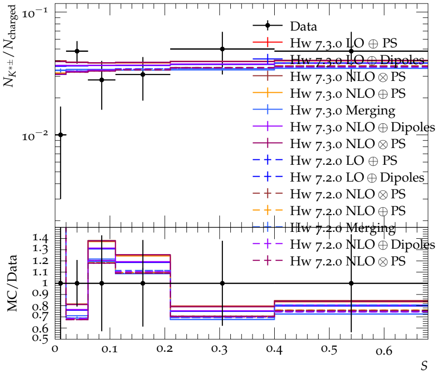
N_{K^{*\pm}}/N_{\text{charged}} vs sphericity at 35 GeV
