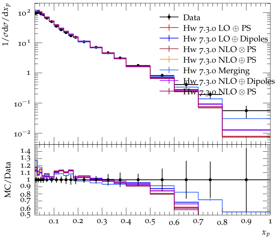
Scaled momentum distribution ( \sqrt{s} = 22 GeV)
