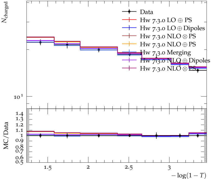
Charged particle multiplicity vs thrust
