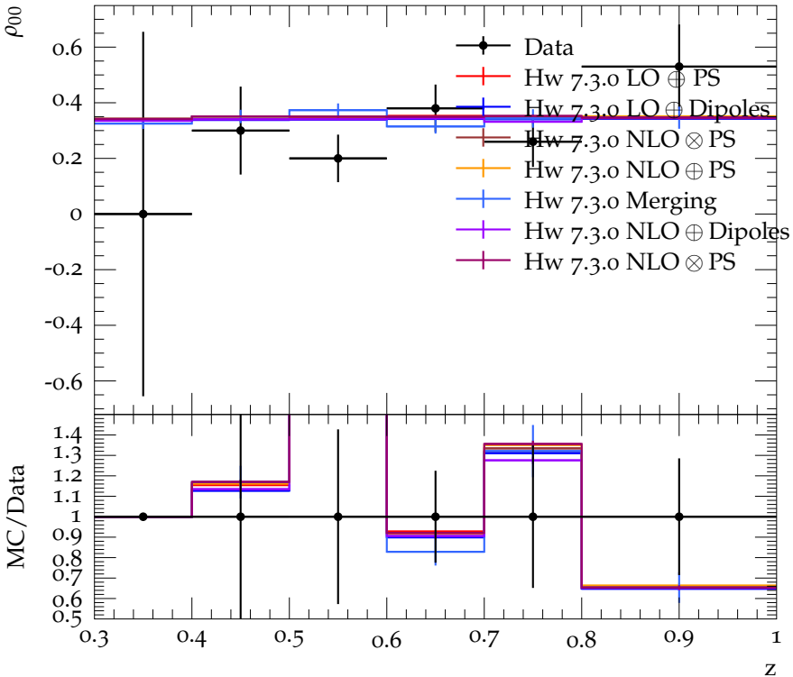
\rho_{00} VS x_E
