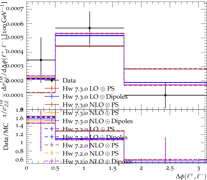
Differential cross-section for ZZ \rightarrow ll\nu\nu vs. \Delta\phi(l^+, l^-)
