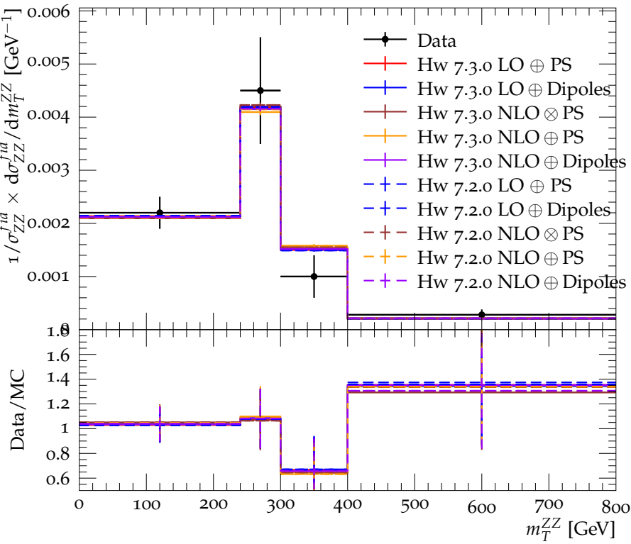
Differential cross-section for ZZ \rightarrow 4\ell vs. M_T^{ZZ}
