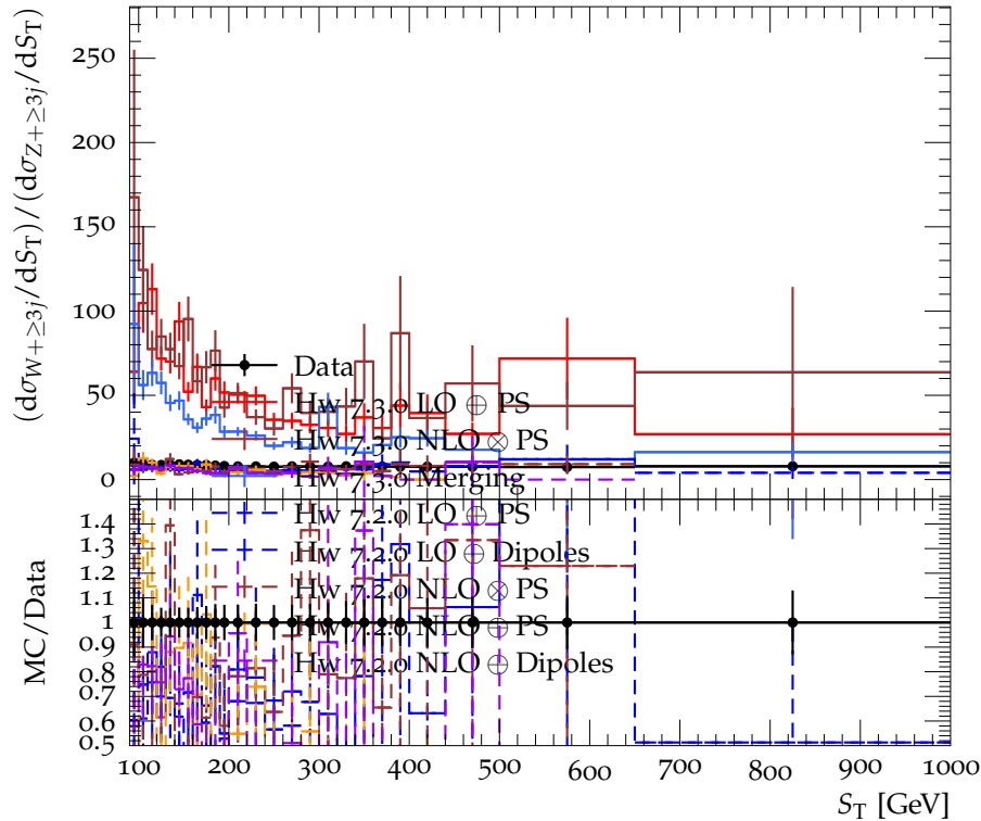
W \rightarrow e\nu/Z \rightarrow ee (MC) vs W \rightarrow \ell\nu/Z \rightarrow \ell\ell (data), dressed level
