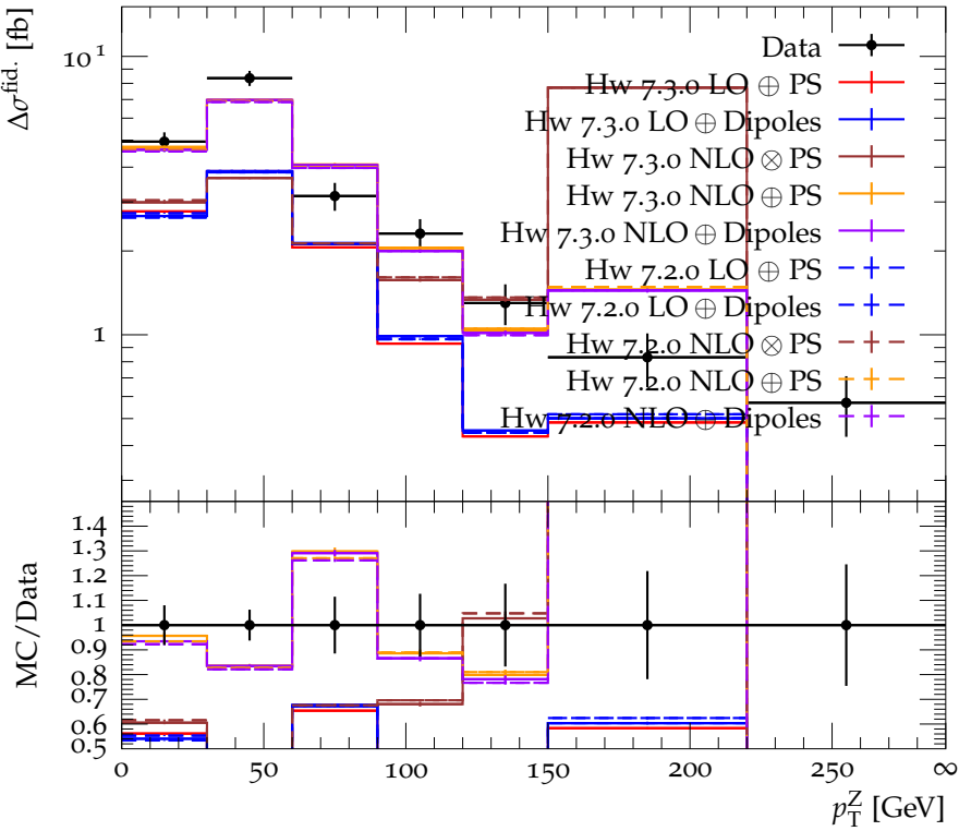
Differential fiducial W^+Z cross section as a function of p_T^Z
