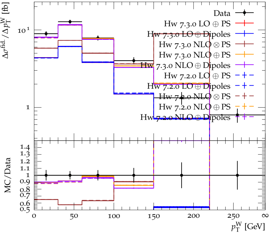
Differential fiducial W^\pm Z cross section as a function of p_T^W
