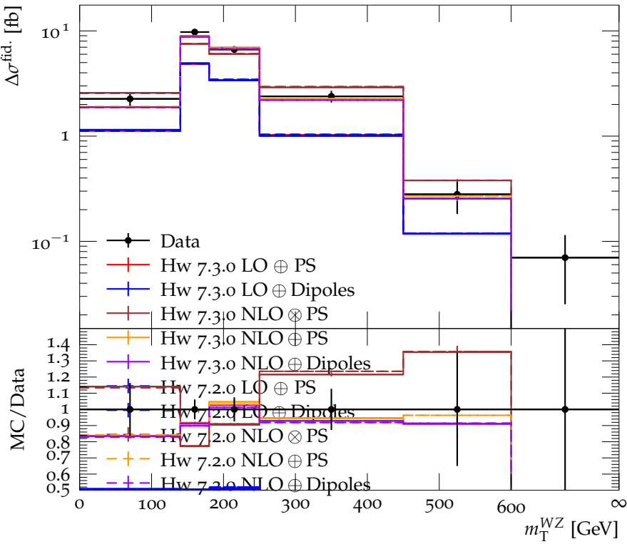
Differential fiducial W^+Z cross section as a function of m_T^{WZ}
