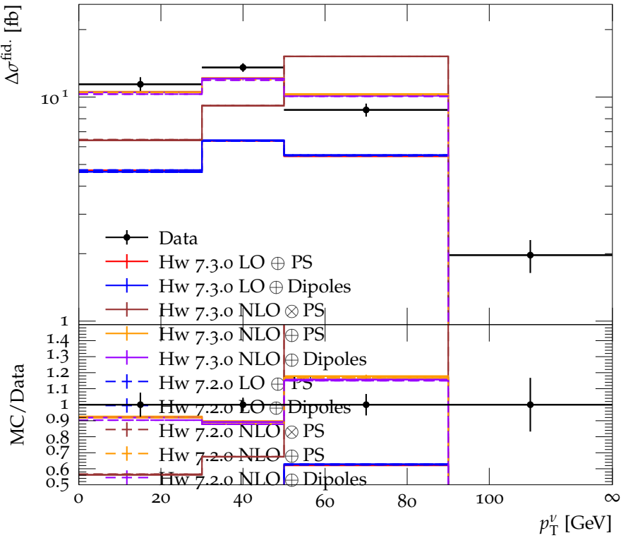
Differential fiducial W^\pm Z cross section as a function of p_T^\nu
