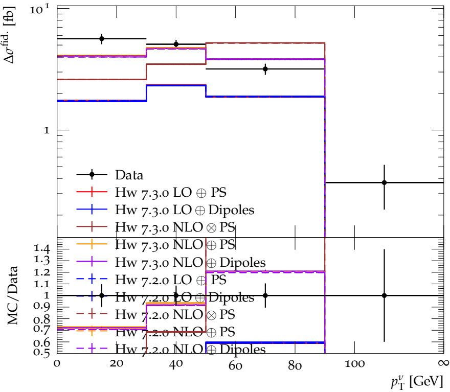
Differential fiducial W^-Z cross section as a function of p_T^\nu
