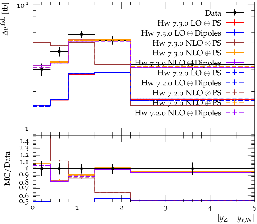
Differential fiducial W^+Z cross section as a function of |yz - y_{e,w}|
