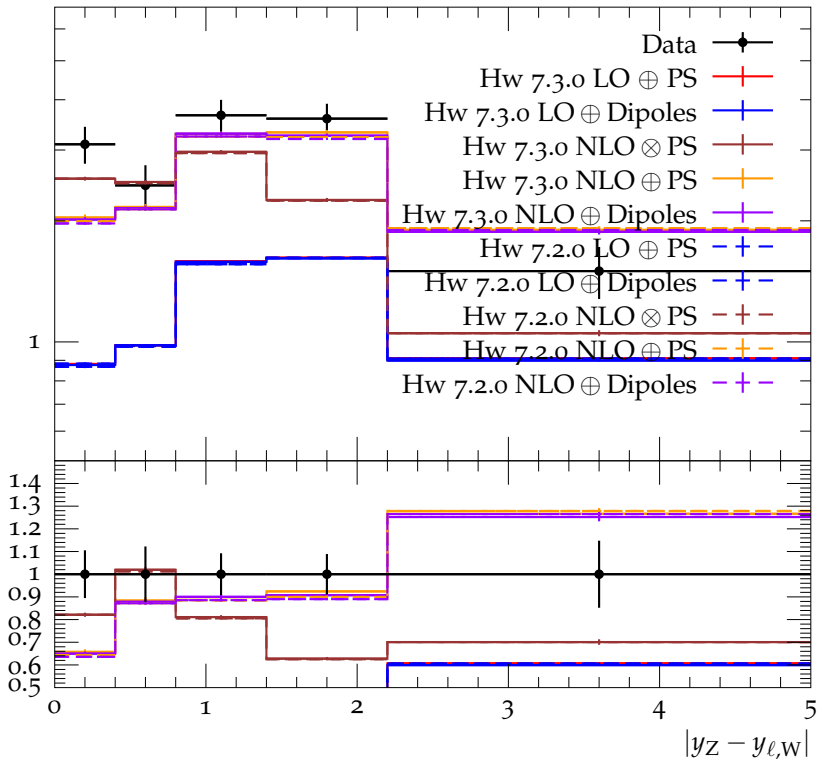
Differential fiducial W^-Z cross section as a function of |yz - y_{\ell,w}|
