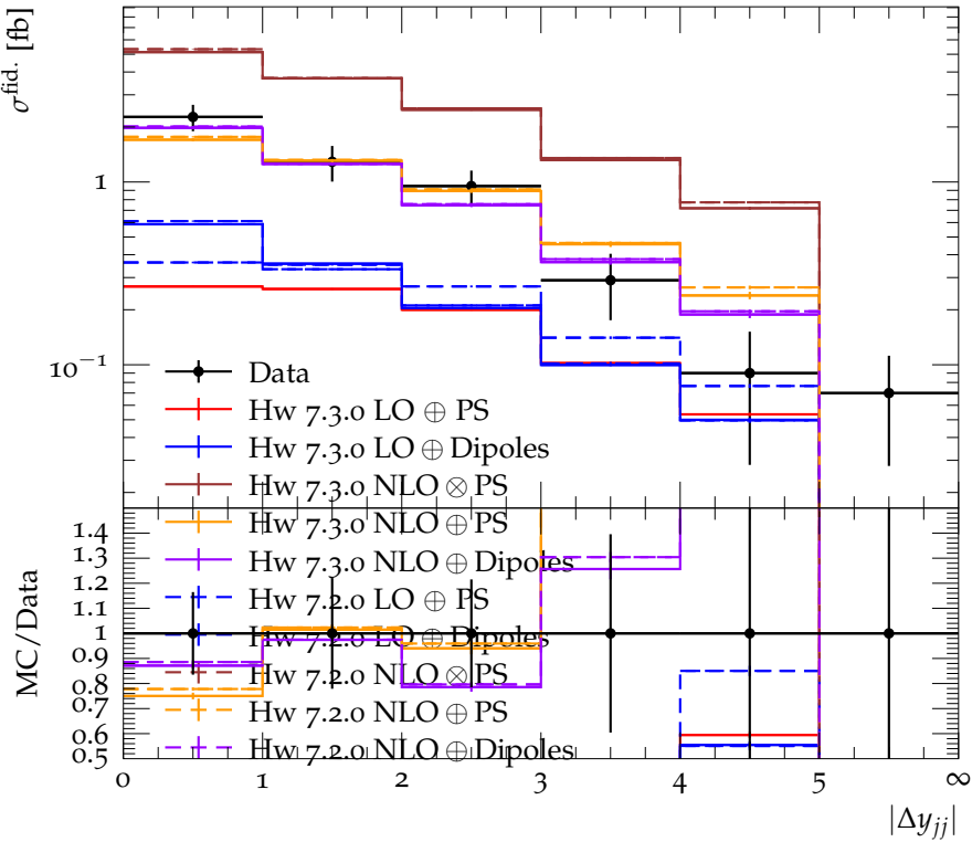
Differential fiducial W^\pm Z cross section as a function of |\Delta y_{jj}|
