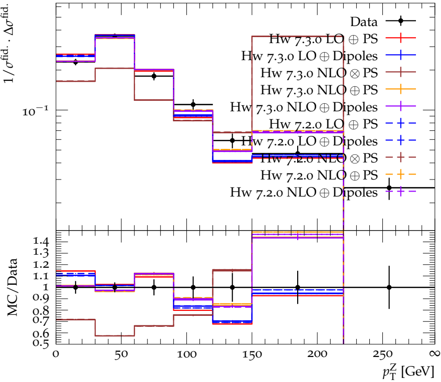
Normalised differential W^\pm Z cross section as a function of p_T^Z
