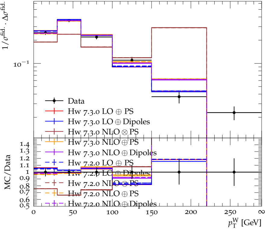
Normalised differential W^\pm Z cross section as a function of p_T^W
