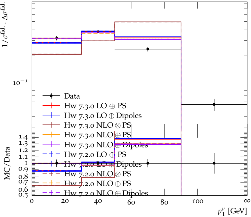
Normalised differential W^\pm Z cross section as a function of p_T^\nu
