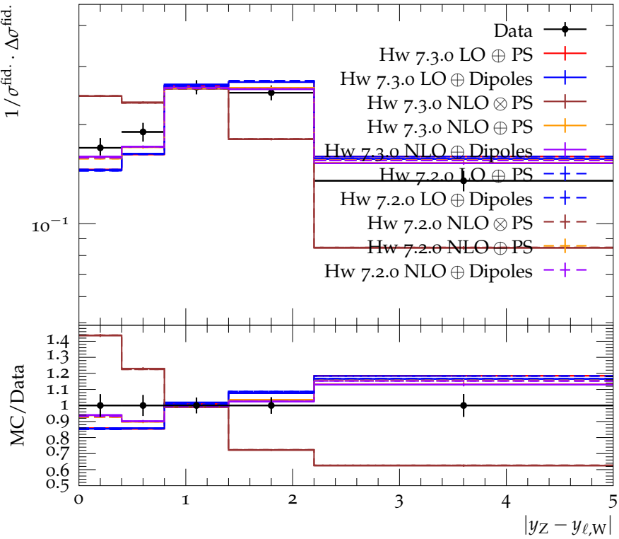
Normalised differential W^\pm Z cross section as a function of |yz - y_{e,w}|
