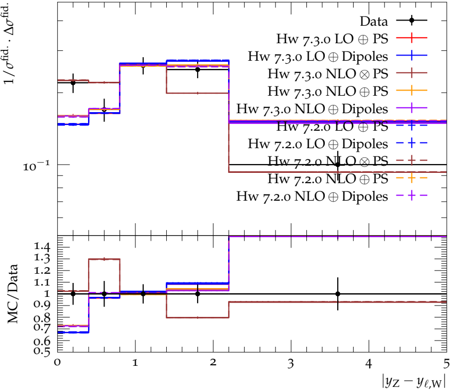
Normalised differential W^-Z cross section as a function of |yz - y_{e,w}|
