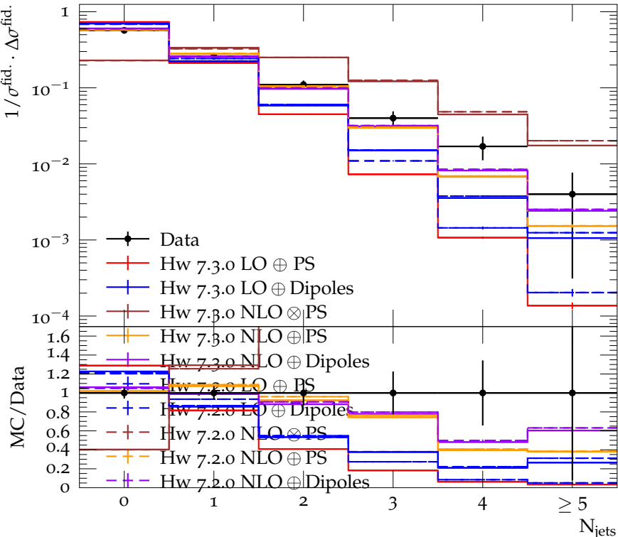
Normalised cross section as a function of the jet multiplicity
