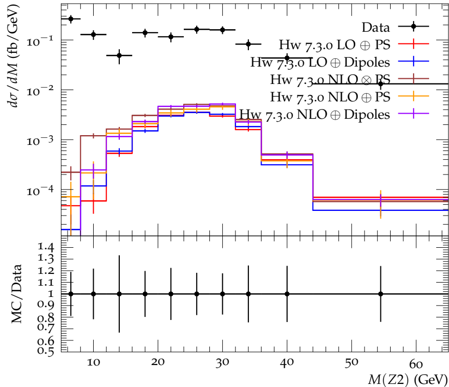
Mass of the second dilepton pair in the H mass region (Max = 59.6)
