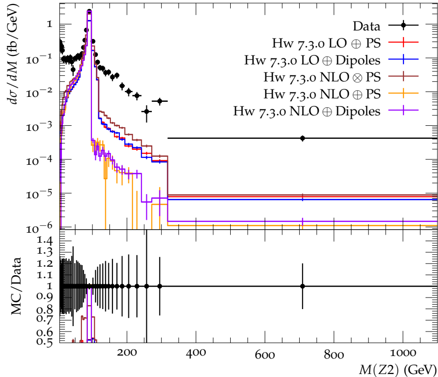
Mass of the second dilepton pair in the ZZ mass region (Max = 1000)
