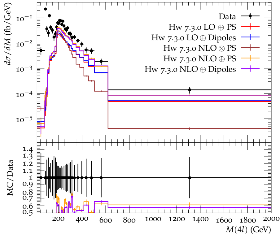
Four lepton mass in fourth p_T^{4l} slice (Max = 1320 GeV)
