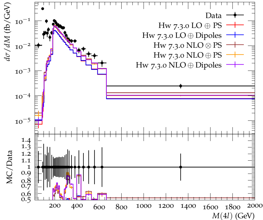
Four lepton mass in first y^{4l} slice (Max = 1710 GeV)
