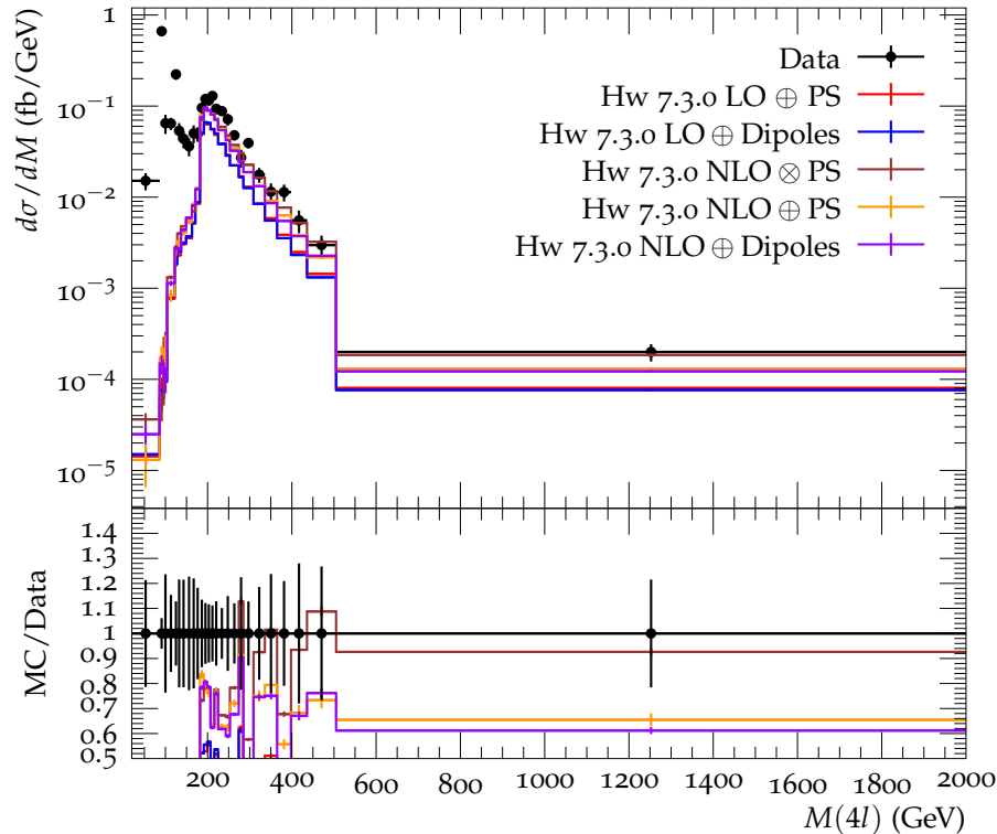
Four lepton mass in fifth y^{4l} slice (Max = 918 GeV)
