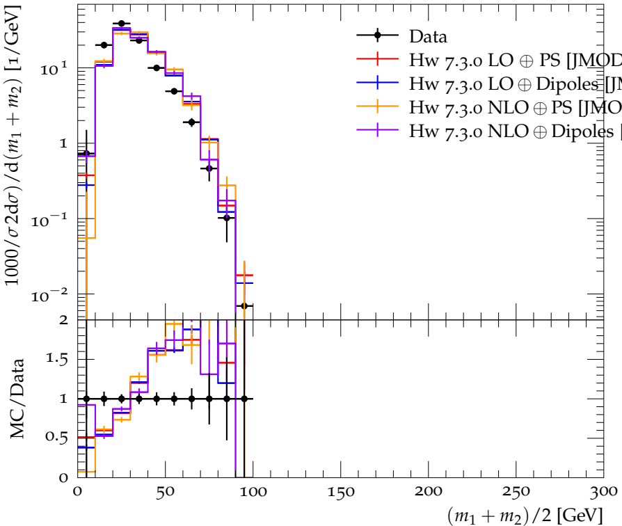
Filtered AK7 W +jets, p_{T,j} = 150\text{--}220 GeV
