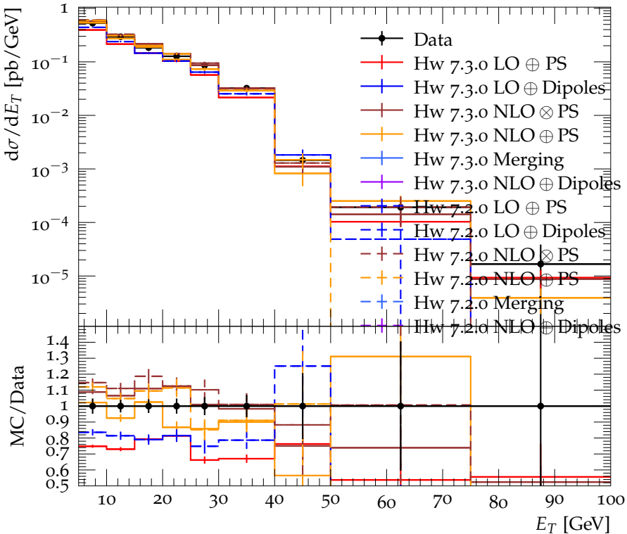
CMS, 7 TeV, Z \rightarrow \mu\mu\gamma , Photon E_T ( q_T < 10 GeV)
