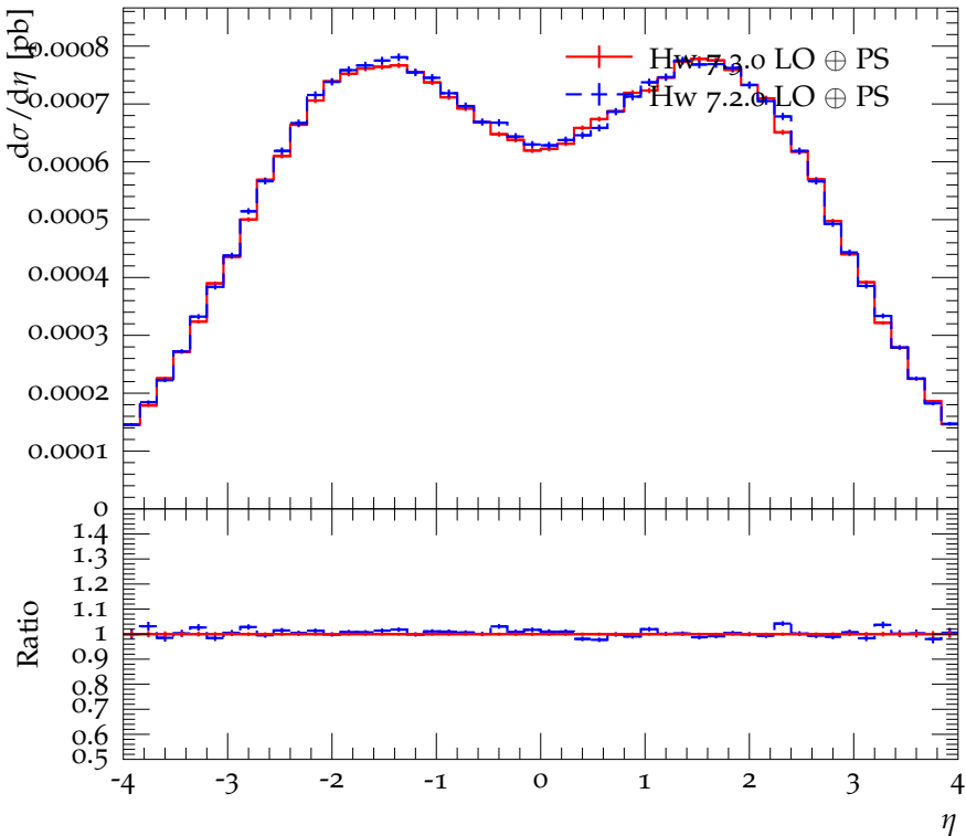
\eta of Higgs candidate from b -jet pair
