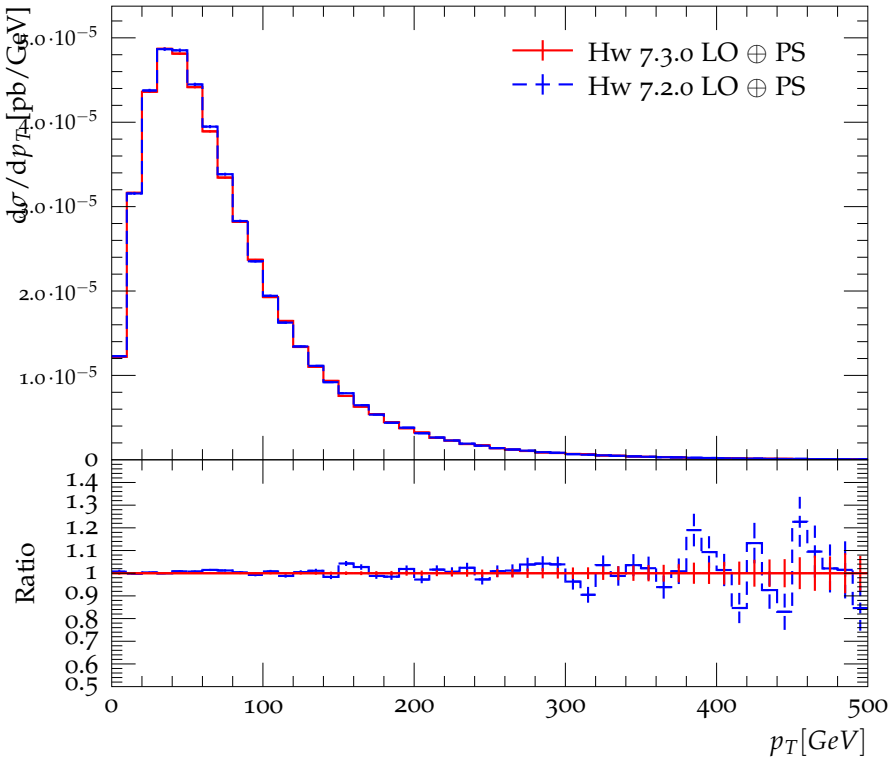
p_T of Higgs candidate from b -jet pair
