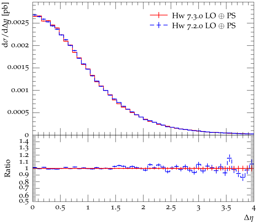
\Delta\eta between Higgs candidate and W
