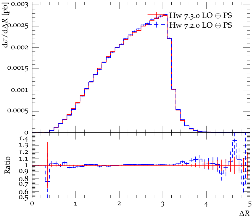
\Delta R between b -jet pair
