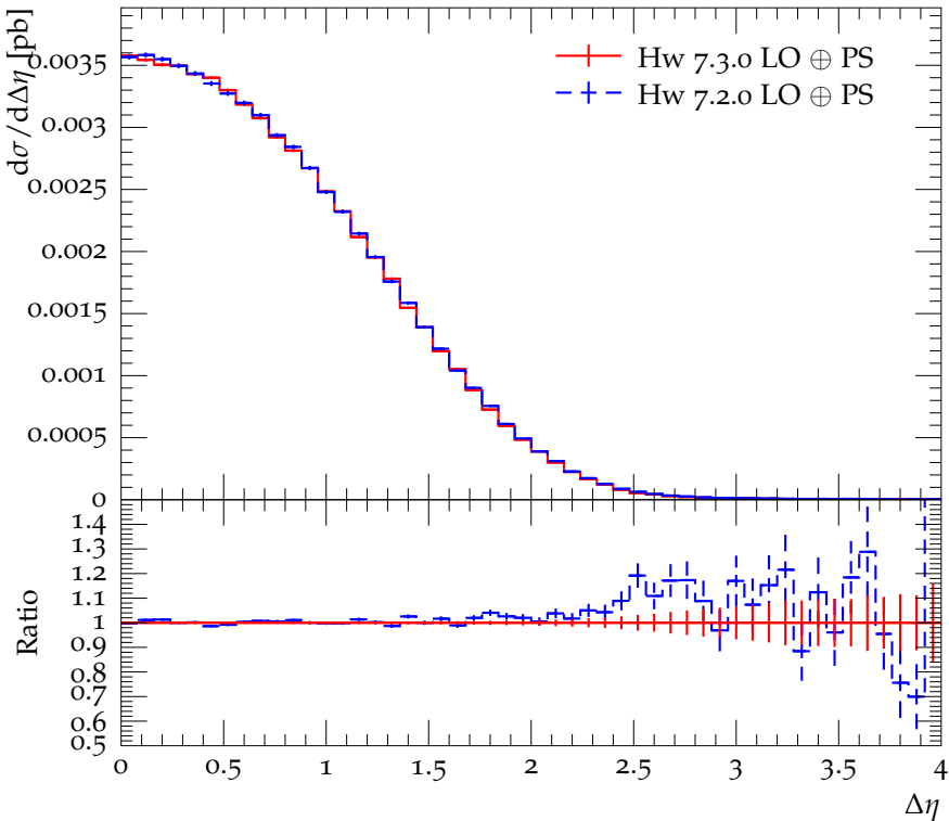
\Delta\eta between b -jet pair
