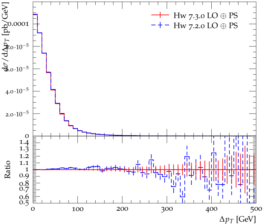
\Delta p_T between b -jet pair
