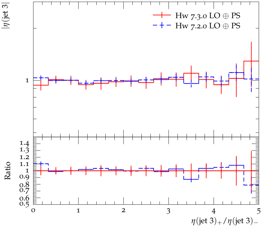
Pseudorapidity \pm ratio of third jet
