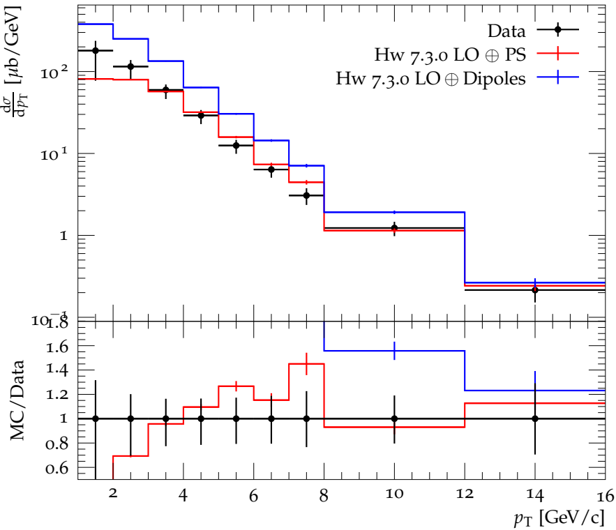
Differential cross section for prompt D^0 production at |y| < 0.5 .
