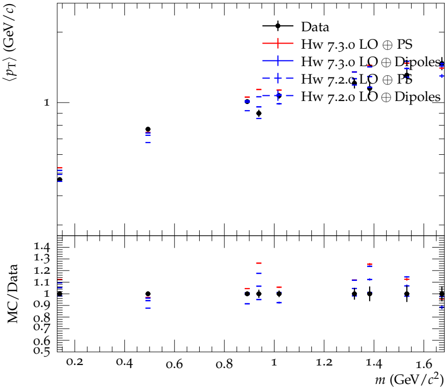
Mean p_T vs mass in INEL pp collisions at \sqrt{s} = 7 TeV in |y| < 0.5 .
