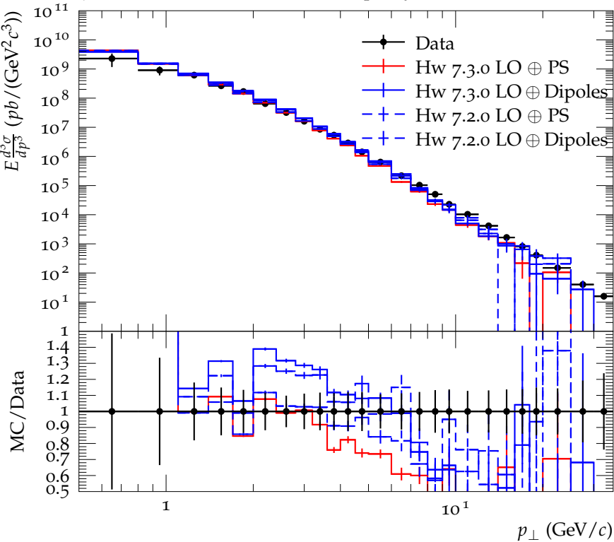
\eta invariant cross section at mid-rapidity at \sqrt{s} = 8 TeV
