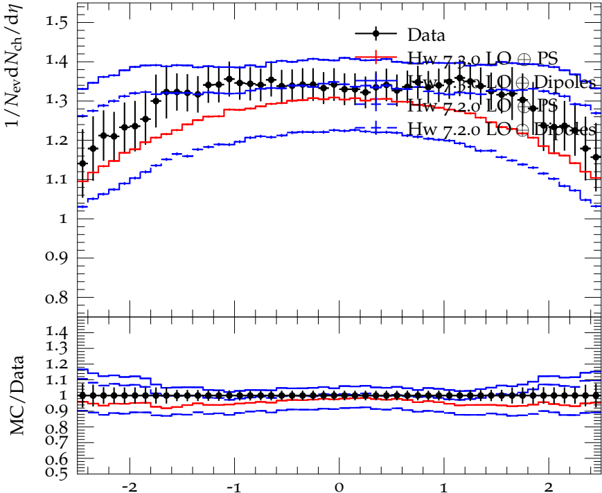
Charged particle multiplicity as function of \eta
