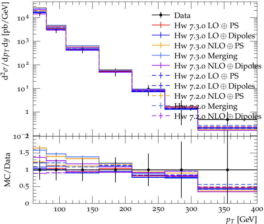
Inclusive jet p_T spectrum for 2.1 < |y| < 2.8 . anti-KT, R = 0.4 .
