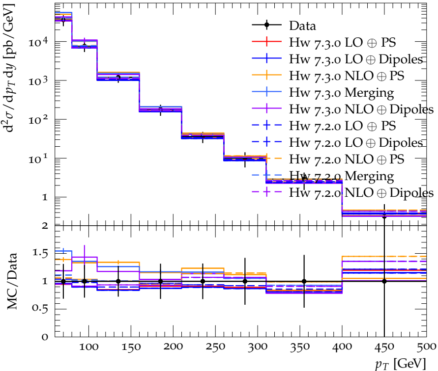
Inclusive jet p_T spectrum for 1.2 < |y| < 2.1 , anti-KT, R = 0.6 .
