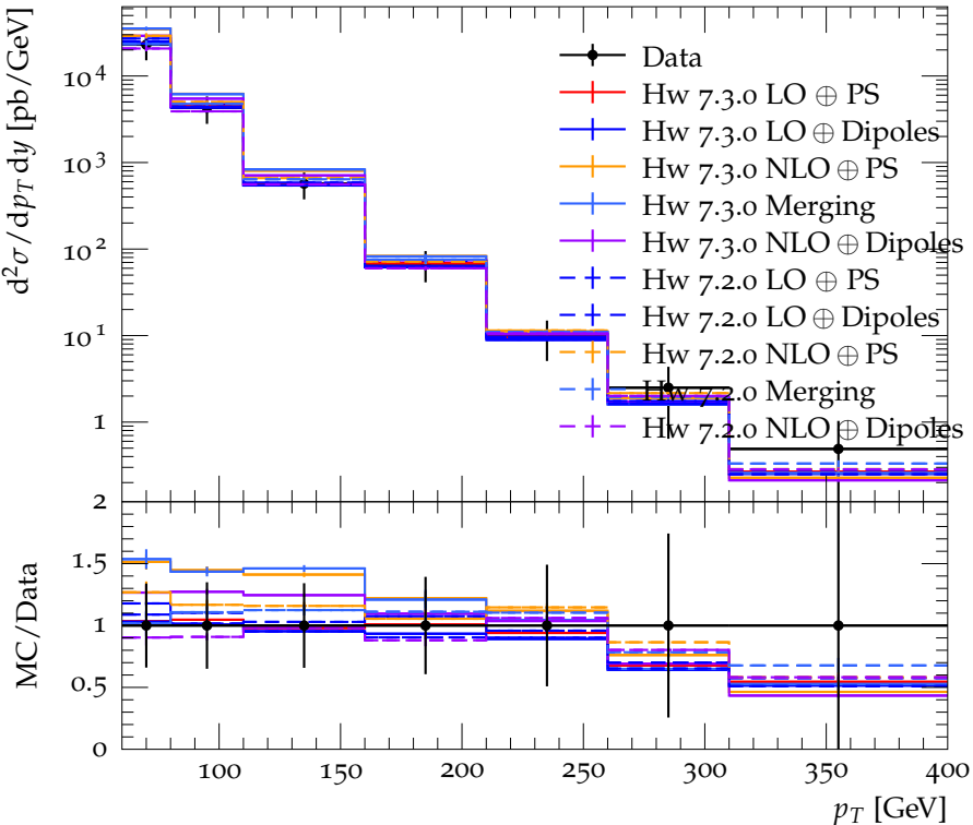
Inclusive jet p_T spectrum for 2.1 < |y| < 2.8 . anti-KT, R = 0.6 .
